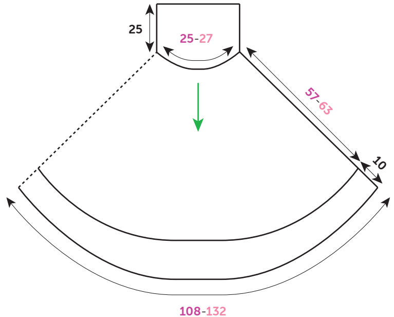
Diagram, measured in cm
